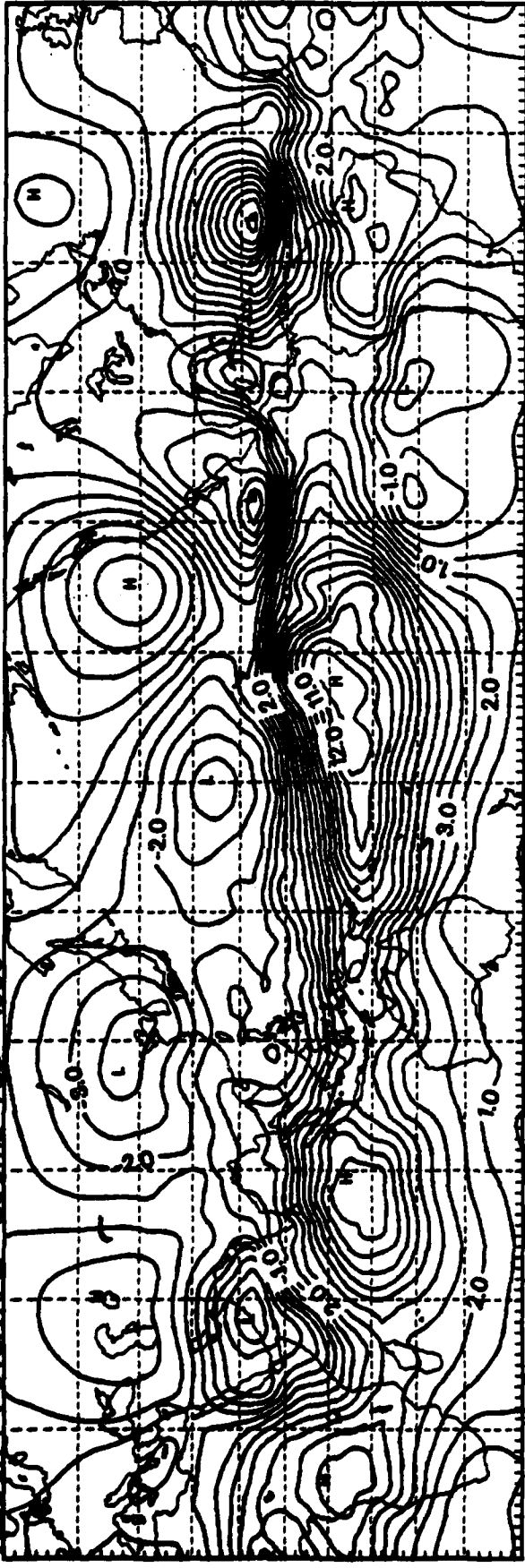
VELOCITY POTENTIAL 200MB FEB 1983
